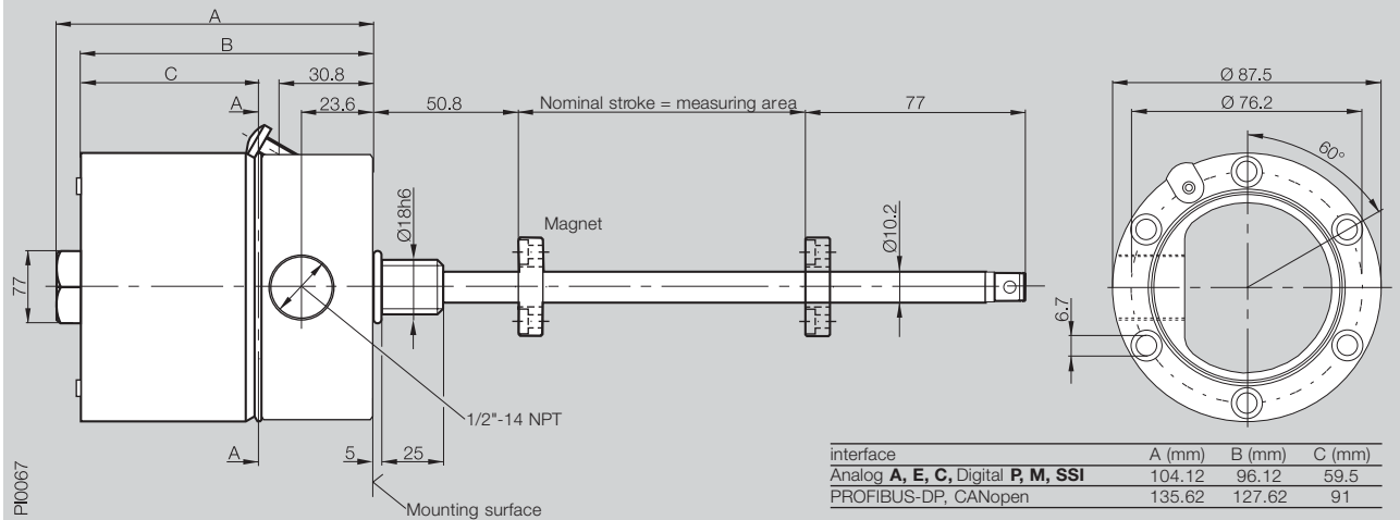
Housing J-DEXC Flange \varnothing 18 mm, PCD \varnothing 76.2 mm
